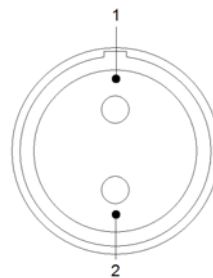
2 PIN LEMO SOCKET VIEW FACING CONTACTS LEMO PART NO. EGG.0B.302.CLL
